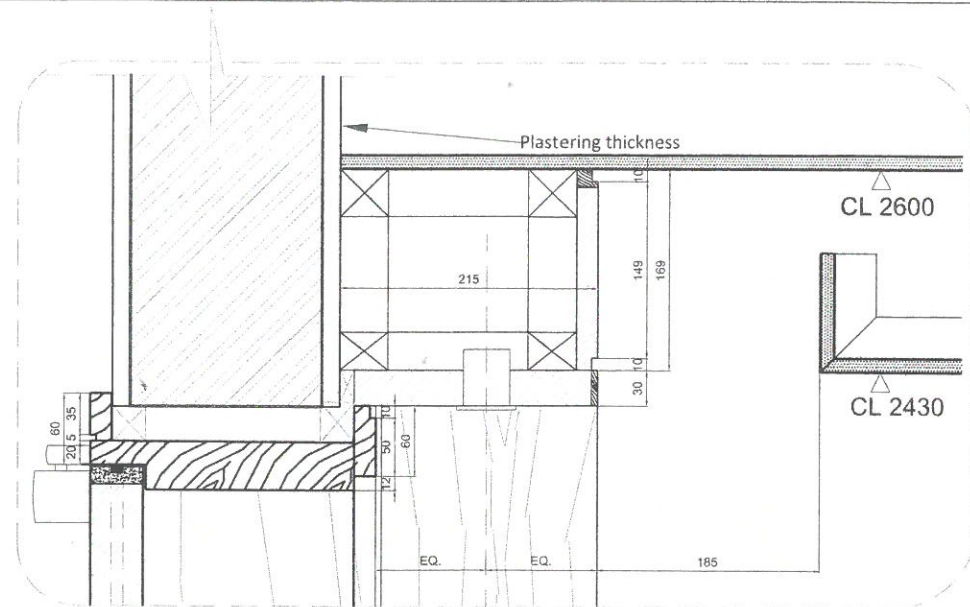
D1 Typical Bulkhead detail
