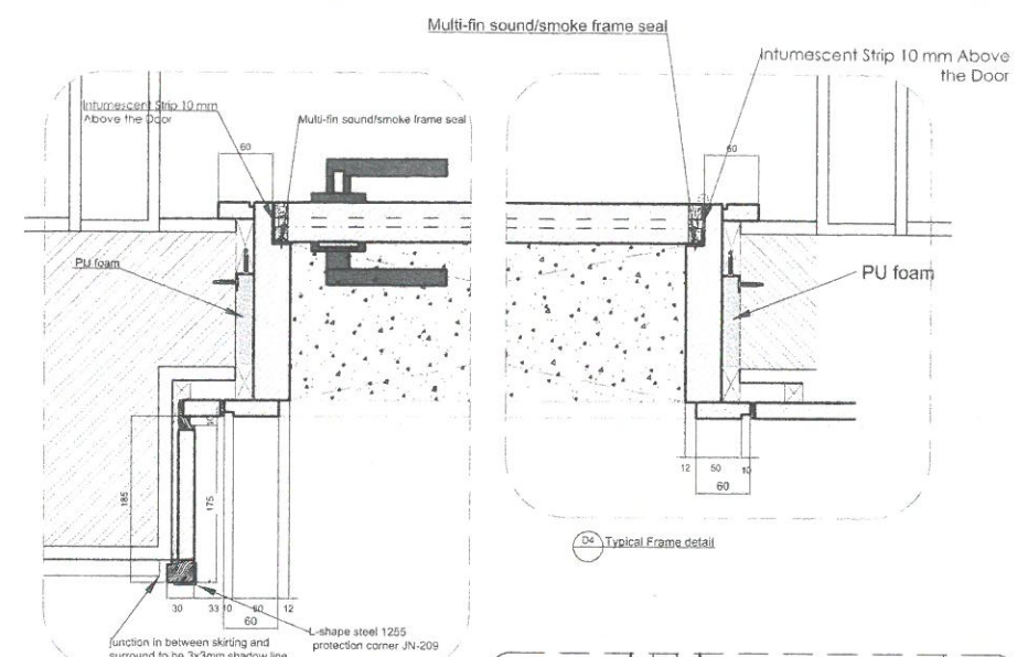
D3 Typical Frame detail
